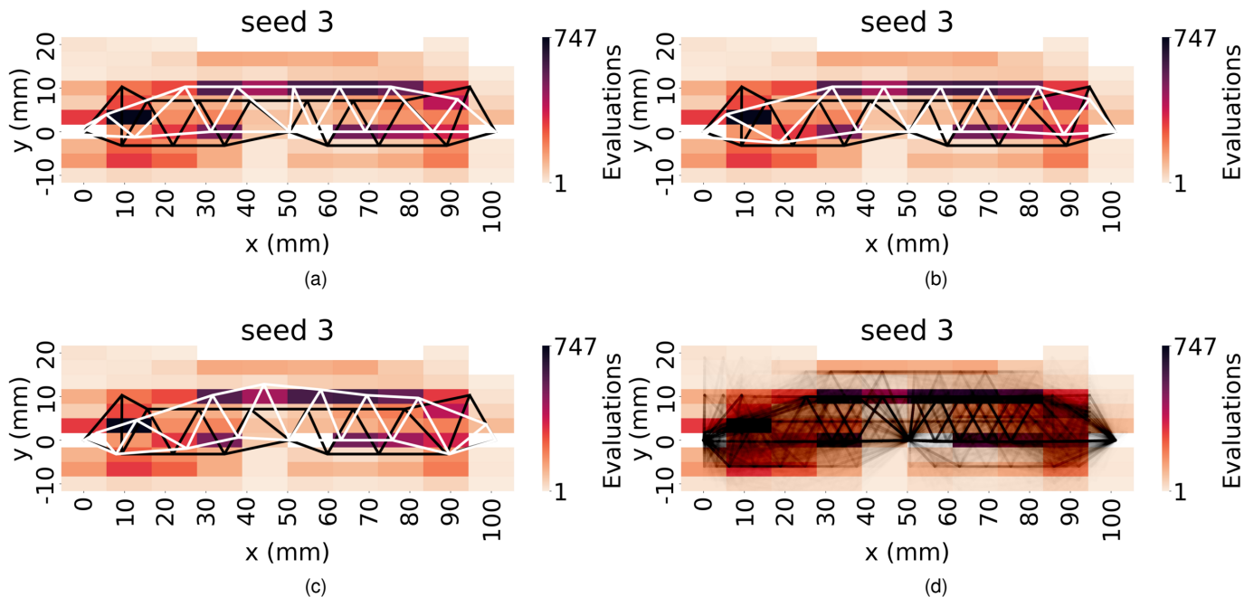
Fig. 5. Figures (a), (b) and (c) represent three examples of solutions (in white) found in the knee region at the Pareto front for seed 3 (in black) each with a coordinate of [371.20, 400.54], [375.54, 379.94] and [384.62, 351.94] respectively where (a) has the lowest volume with the highest deflection and (c) has the highest volume with the lowest deflection. Figure (d) illustrates all the structures at the last generation for all the replicates. The colour of the cell represents the number of solutions found with a vertex at that coordinate at the generation.
