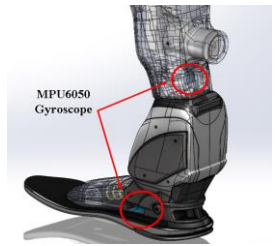
Fig 5: Position of gyroscope & accelerometer (MPU6050 Gyroscope) in E-Leg
